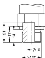
G1/2" open port DIN 3852 (up to 40 bar)
