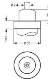
cable outlet, cable with ventilation tube (IP 68) 6
