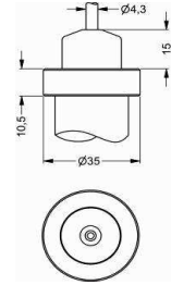
cable outlet with PVC cable (IP 67) 5
