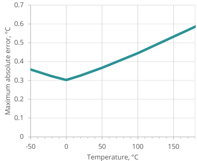
Sensor accuracy 3
