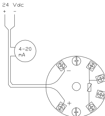
Temperatur transmitter
