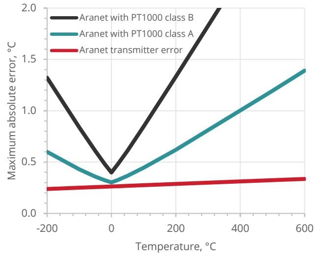
Sensor accuracy 2
